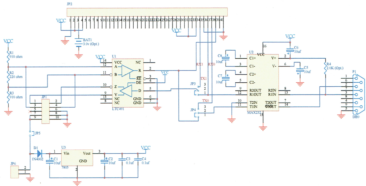
Figure 1 - Z232-485 Converter Board Schematic
